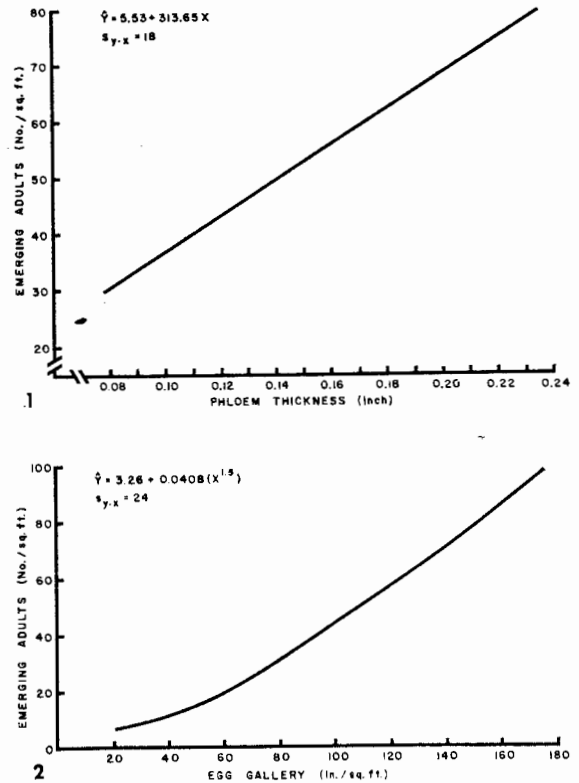
FIG. 1, 2.—Relation between number of emerging brood adults of the mountain pine beetle and thickness of lodgepole pine phloem (Fig. 1) and inches of egg gallery made by parent adults (Fig. 2).
