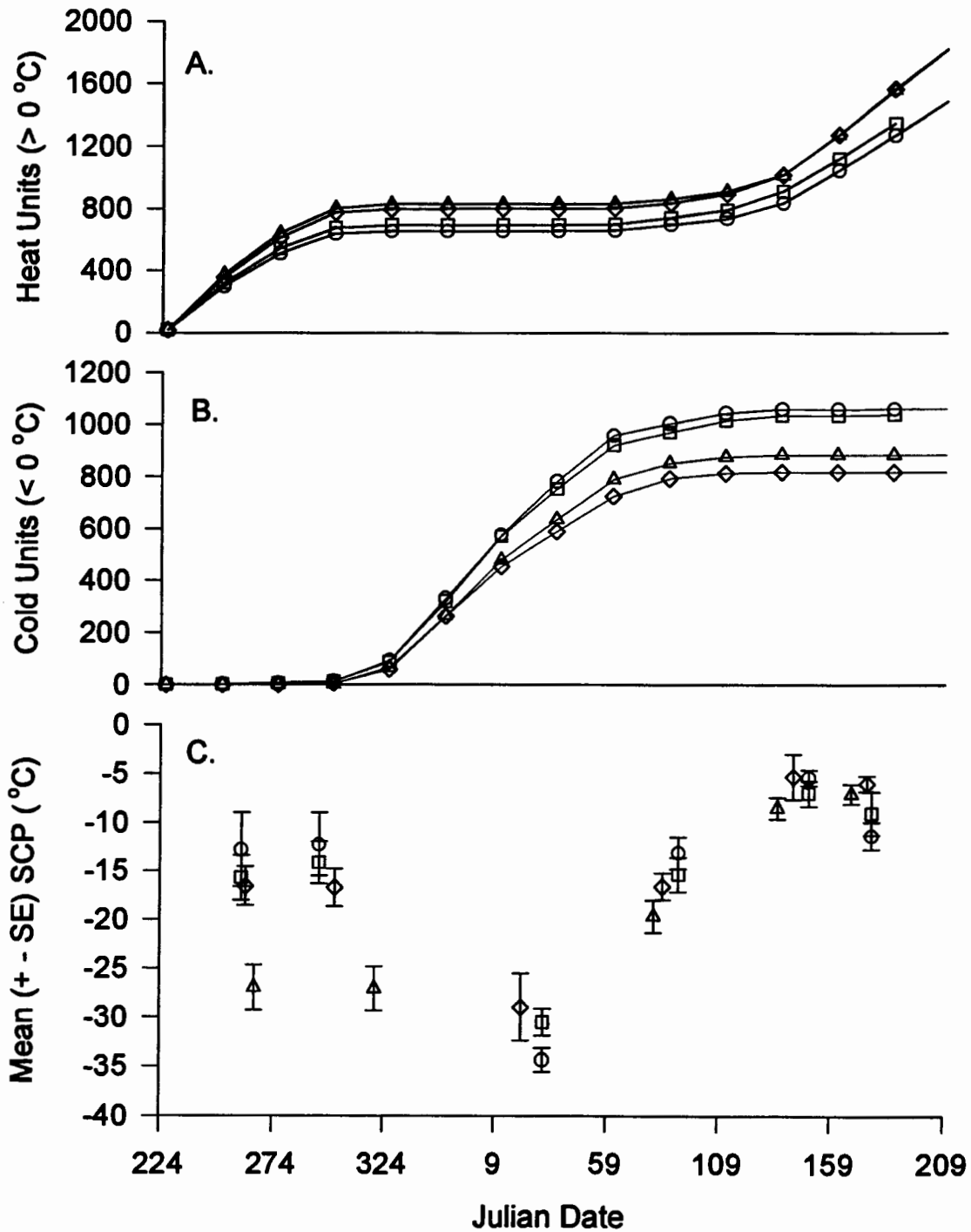
Fig. 3. (A) Accumulated heat units (>0°C) and (B) accumulated cold units (<0°C) at 4 sites in 1992-1993 and (C) associated mean supercooling points (SCP) (°C) and standard errors. Sites: ○, Ranch; □, Galena; △, Logan; ◇, Moose.
