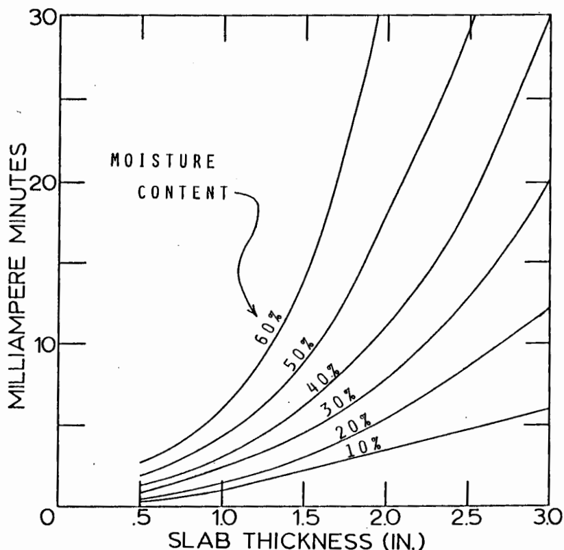
Figure 2.--X-ray exposure curves for wood and bark slabs (Lodgepole pine) of different thickness and moisture content when the X-ray unit is operating at 25kV, 5mA, using a 51-cm (1 inch = 2.54 cm) target film distance (from Arman and Rasmussen, J. Econ. Entomol. 62:631-634, 1969).
