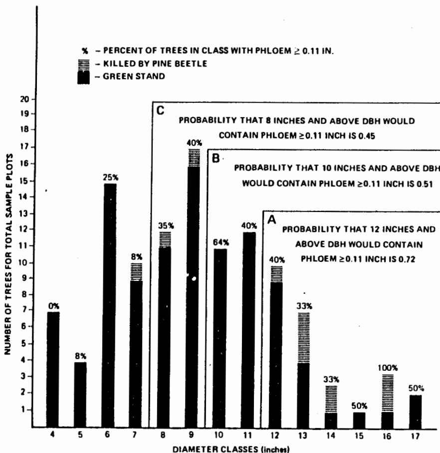
Figure 4. Buffalo Peak stand. Land manager's alternatives: A, remove host trees 12 inches dbh and larger; B, remove host trees 10 inches dbh and larger; C, harvest in this case would approximate a clearcut because most of the trees are in the larger classes.
