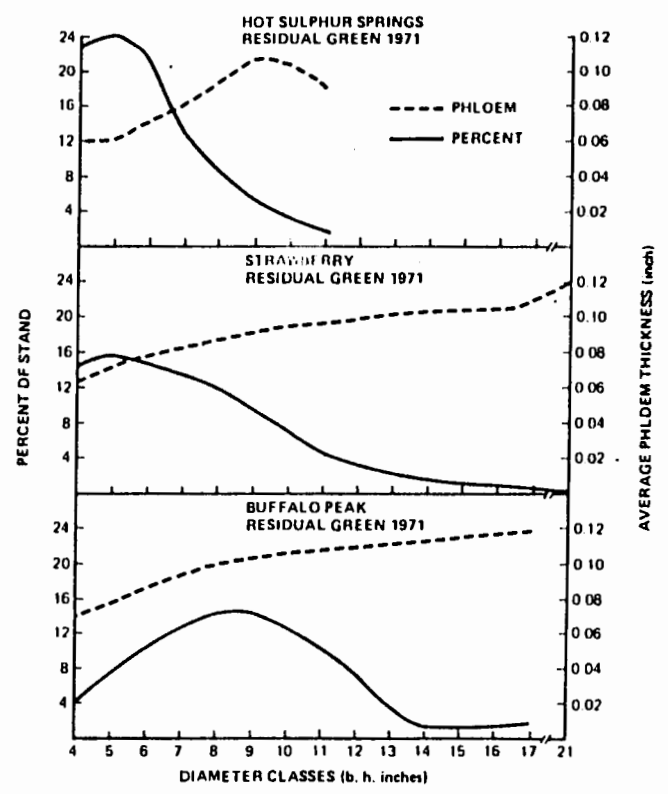
Figure 1. Relationship between diameter distribution within stands and phloem thickness distribution among diameter classes for green trees.
