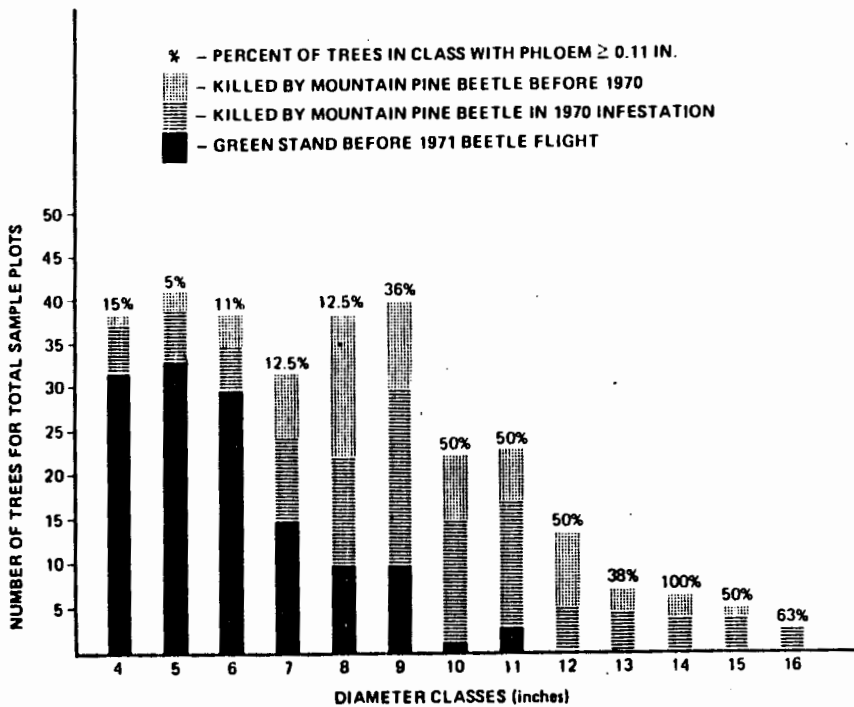
Figure 2. Hot Sulphur Springs stand after 5 years of mountain pine beetle activity.
