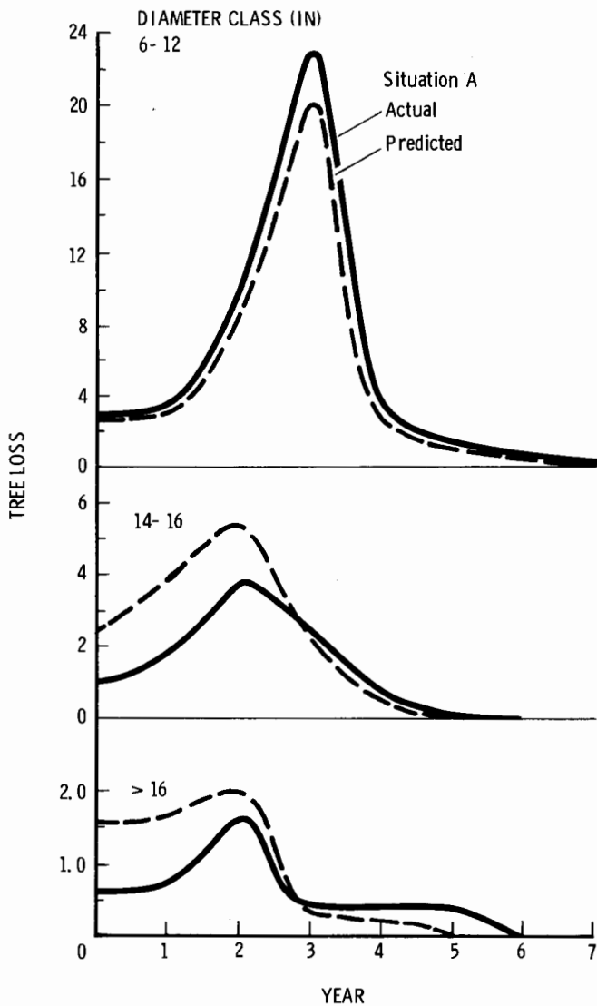
Figure 2.—Predicted versus observed tree loss by year based on q_t , by grouped tree diameter classes and total stand (Situation A, Klein and others 1978).
