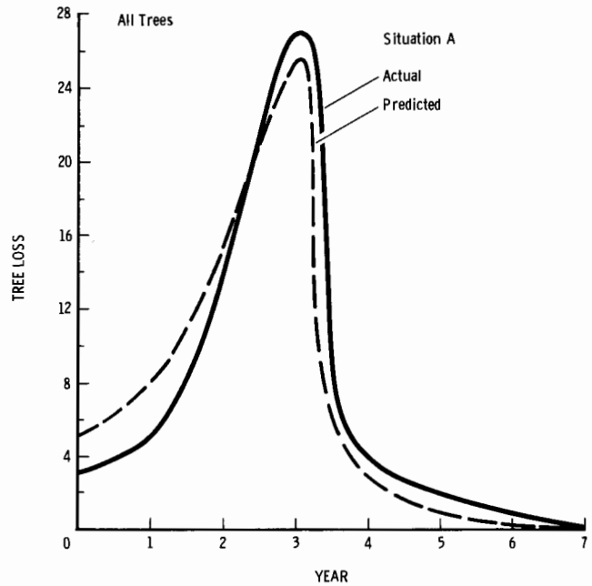
Figure 3.—Predicted versus observed tree loss by year for total stand based on q_t (Situation A, Klein and others 1978).
