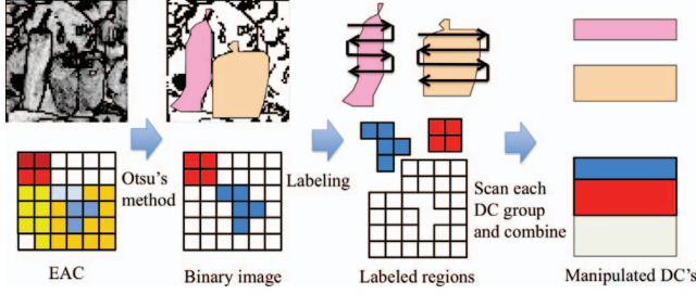
Fig. 2. Flow of operations in encoding DC coefficients
