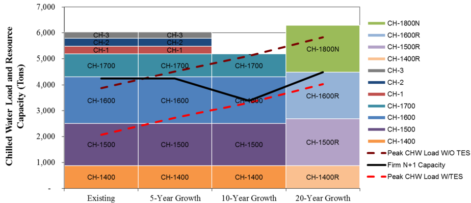
Figure 6-2: Base Case – Chiller Asset Roadmap
