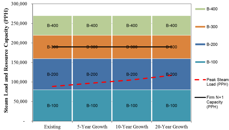
Figure 6-1: Base Case – Boiler Asset Roadmap
