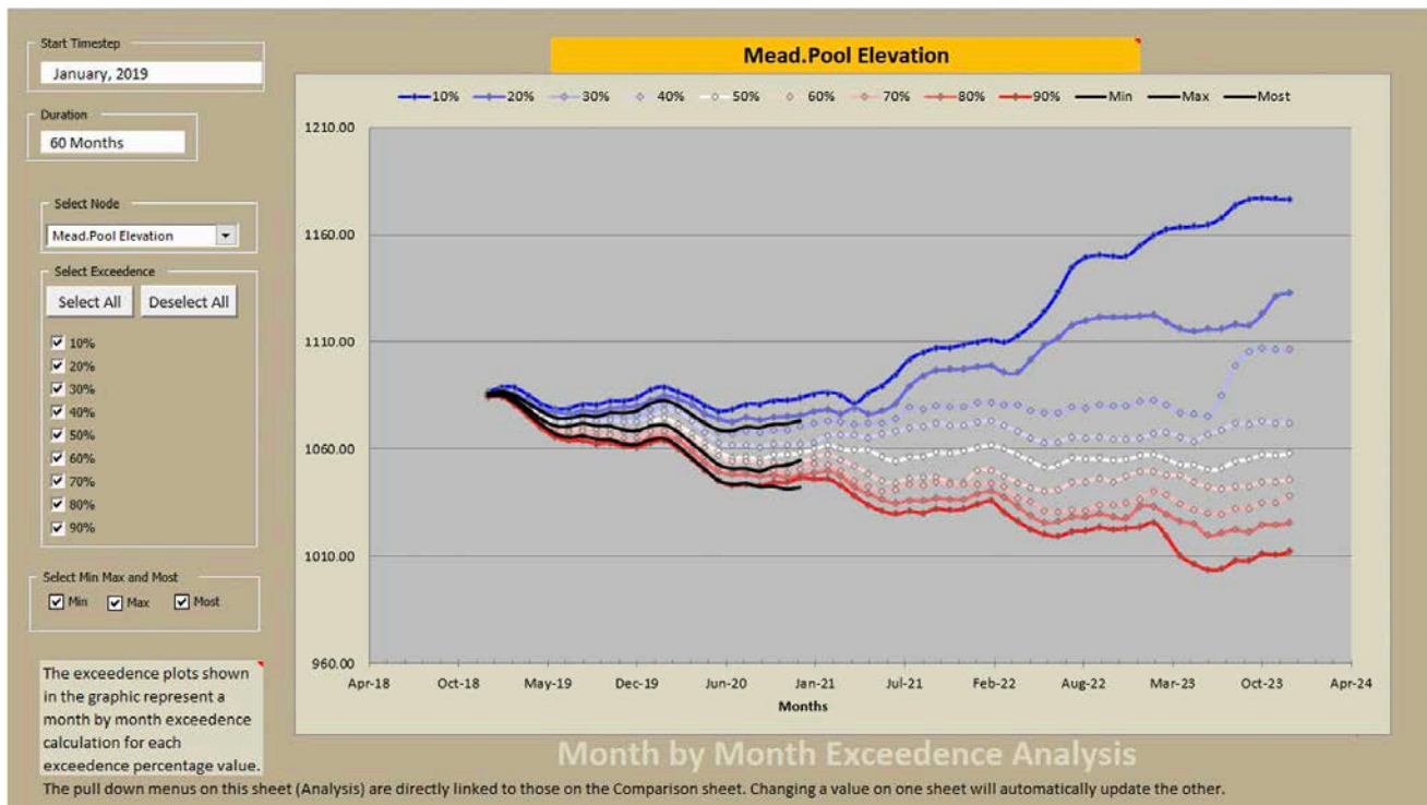
Figure 8. Projected Lake Mead elevation for the next 5 years under different probability of exceedance (from Colorado River Basin MTOM Technical User Guide for Stakeholders, version 2.0).
