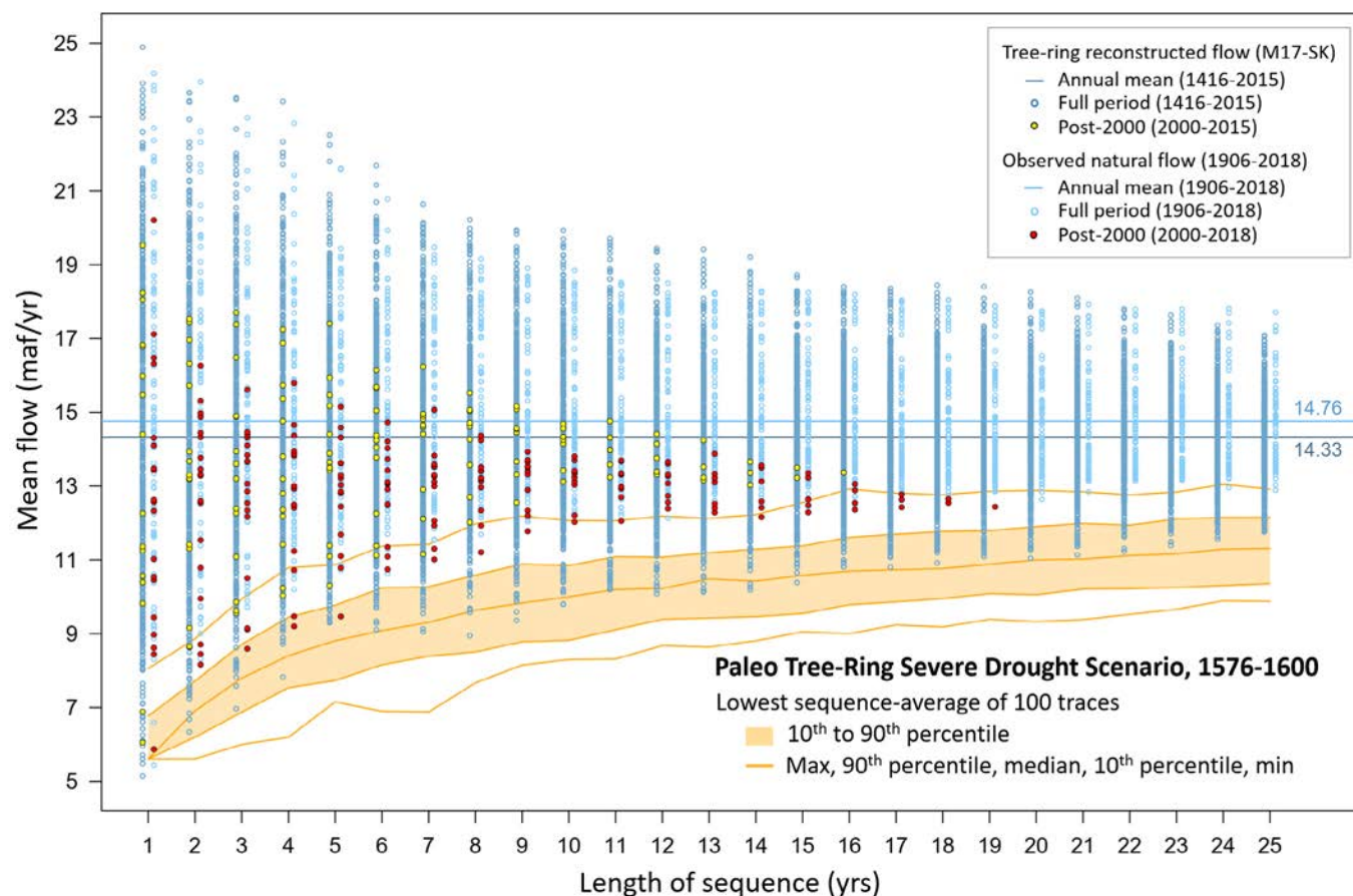
Figure 26. The lowest sequence-average of paleo tree ring severe drought in comparison with observed and tree ring reconstructed flows.
