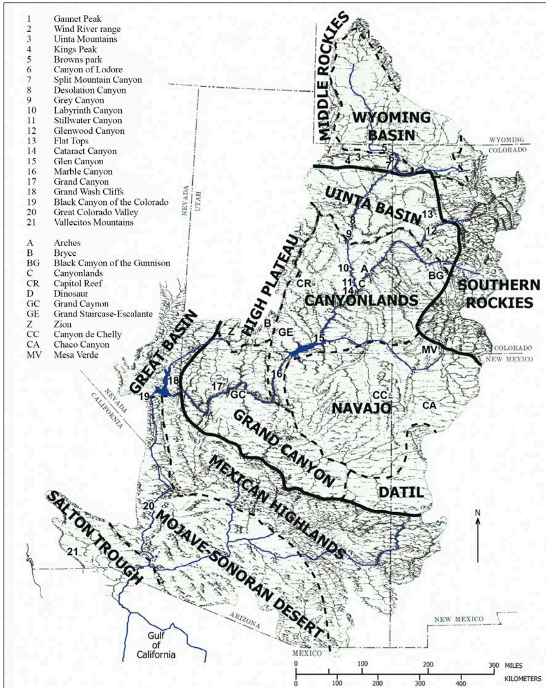
Figure 2. Map showing the subdivisions of the three physiographic provinces of the Colorado River watershed. The Rocky Mountains are in the north and east; the Colorado Plateau is in the center of the watershed, and the Basin and Range is to the south and west. The delta of the Colorado River is in the Salton Trough (adapted from Hunt, 1969; and physiographic divisions are from Graf, 1987).
