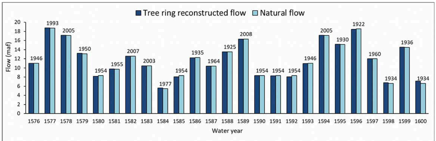
Figure 21. Nearest year of historic natural flow to tree-ring reconstructed flow at Lees Ferry. X axis represents water years of the tree-ring reconstructed flow and the numbers above the bars represent the “parallel” years in the natural flow.
