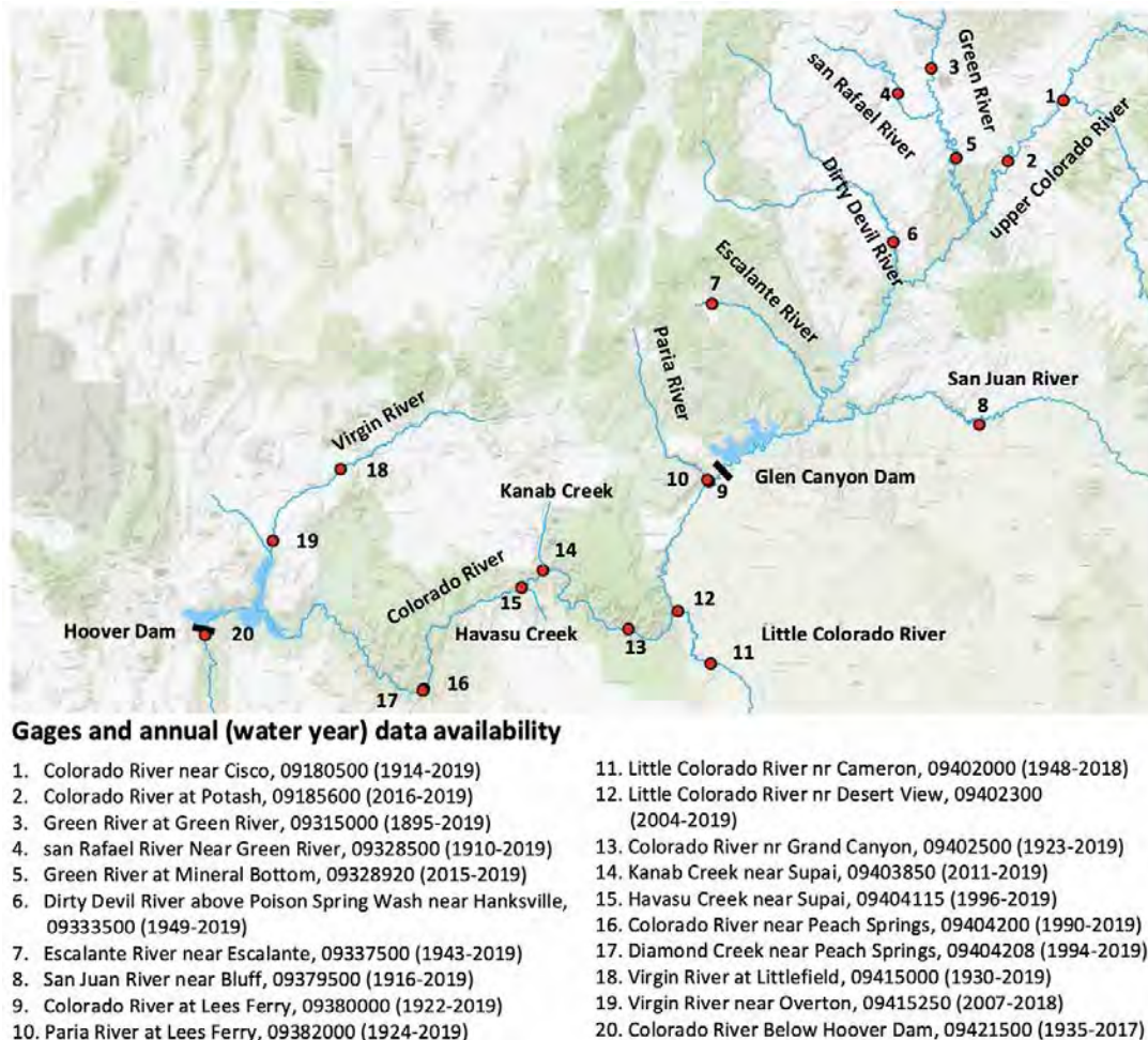
Figure 1. Map showing stream-flow gages and data availability. Each number corresponds to a gage whose official USGS number is listed, along with the period of availability of annual flow data.
