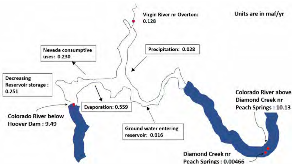
Figure 8. Water budget components for Lake Mead between March 2010 and February 2015. The width of each line is proportional to that river's annual flow.
