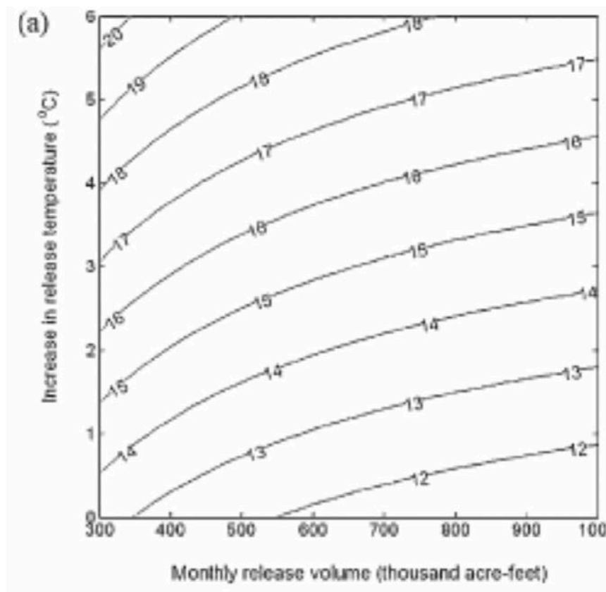
Figure 31. Graph showing predicted temperature near RM 61 as a function of the temperature of the water released from Lake Powell and the monthly volume of those releases. Values shown on contour lines are the predicted water temperature, in C, near the confluence of the Colorado and Little Colorado Rivers. Values on the x axis are the monthly volume of water released from Lake Powell. Values on the y axis are degree of warming of reservoir releases greater than typical releases of 48F (9C), in 1C (1.8F) increments. Simulations are for typical summer conditions where mean daily air temperature is 79F (Wright et al. 2008).
