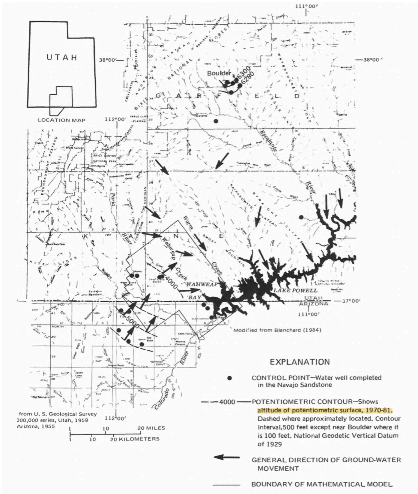
Figure 21. Map showing approximate potentiometric surface and general direction of movement of water in the Navajo sandstone (Thomas, 1986, fig. 6).
