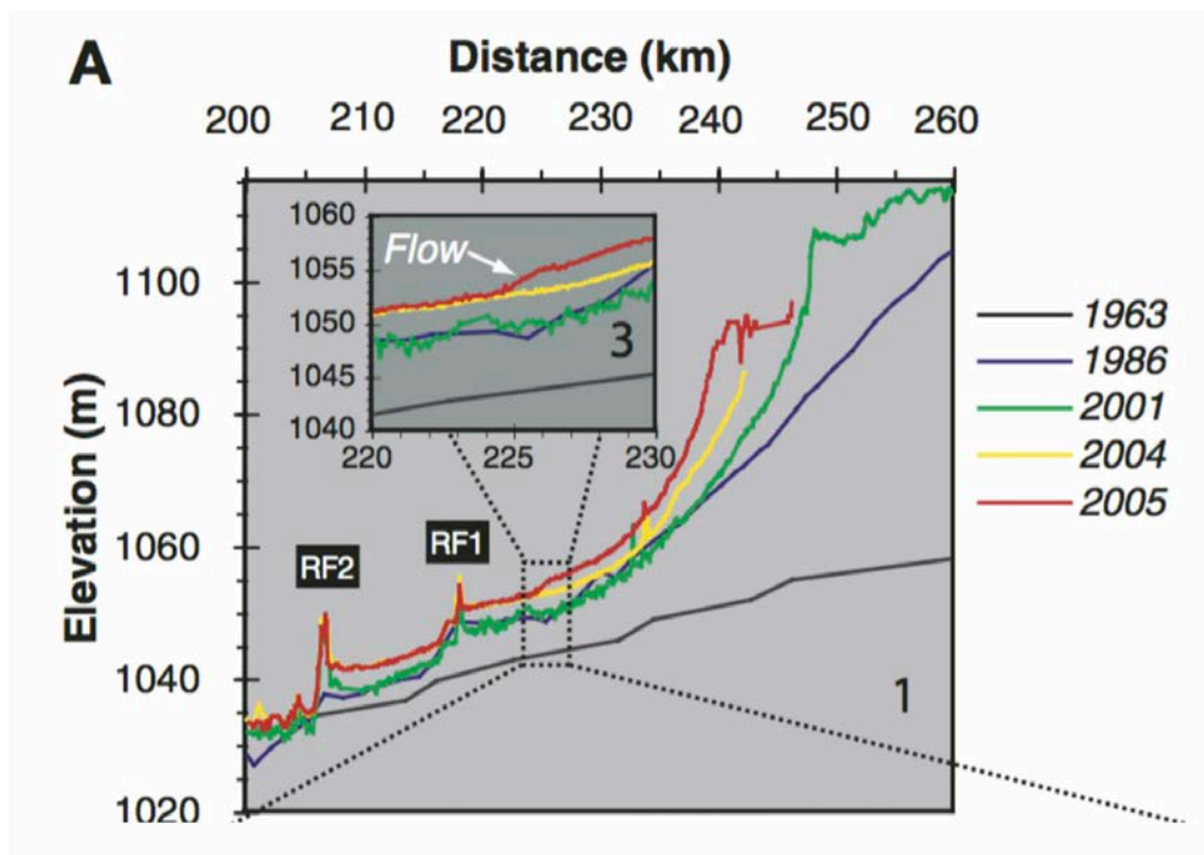
Figure 29. Graph showing the bathymetric profile of the Colorado River delta at different times (Pratson et al., 2008, Fig. 3A). The distance of 240 km shown on this graph is equivalent to a point 150 miles upstream from Glen Canyon Dam shown on the graphs of Majeske (2009).
