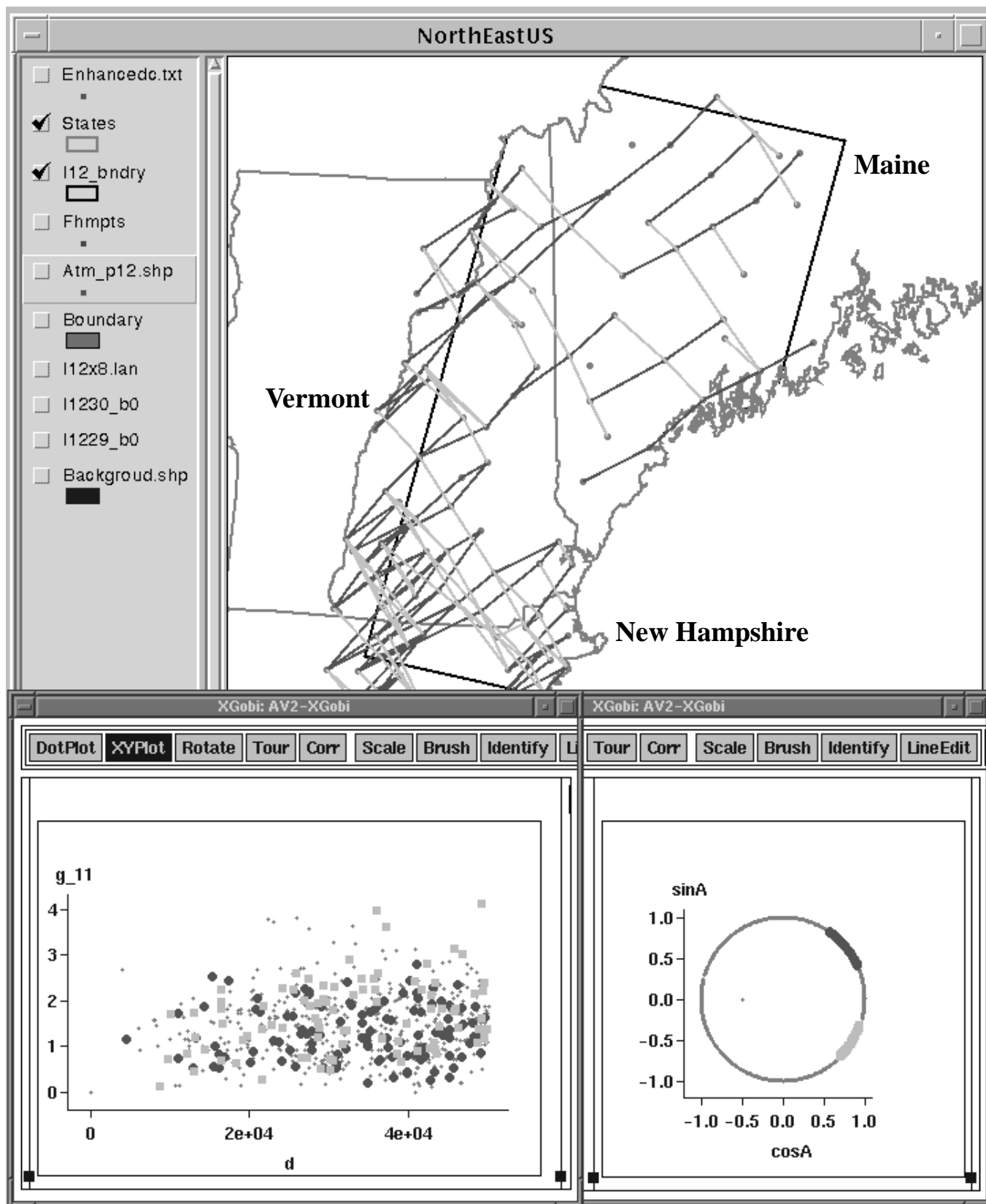
Figure 3: Variogram-Cloud Plot (bottom left), Angle between Locations (bottom right), Map View of Sampling Sites in the Northeastern United States (top).
